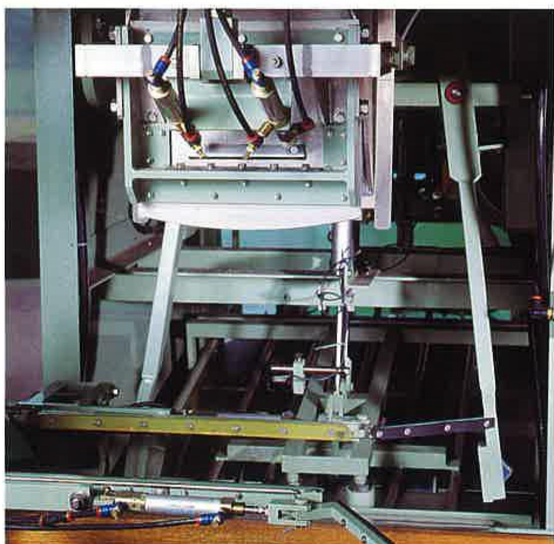
Bag Clamp/Filling Section
